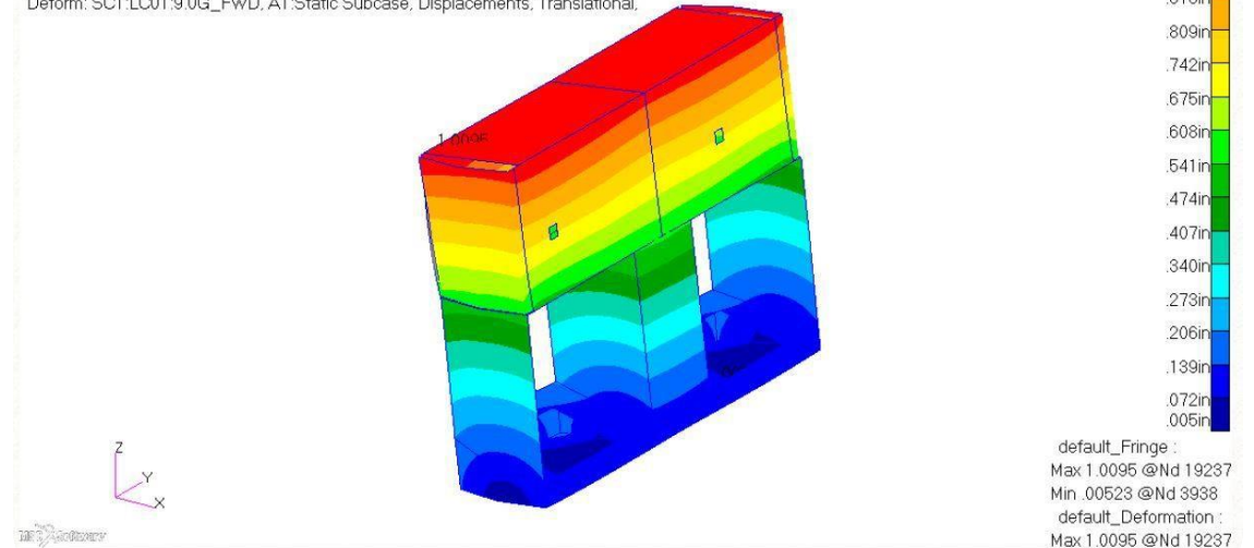
Figure 7 – LC01: 9.0g Forward Case [Maximum Deflection = 1.010in, 25.7mm]
